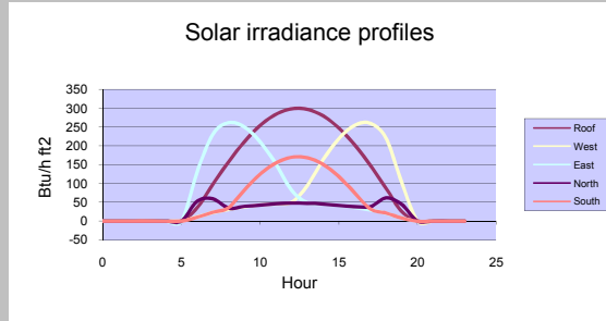
Design daily temperature and solar irradiance profiles
